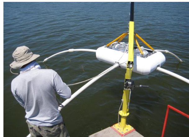
Figure 4. Deployment of SMMT system during marine EM survey from the pontoon boat.
