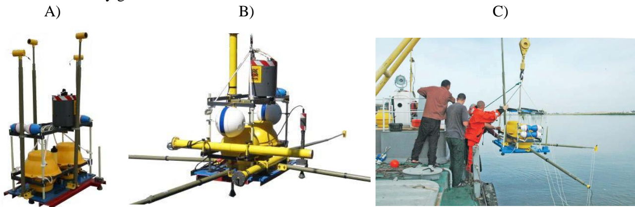
Figure 3: Marine EM receivers for coastal shelf exploration; A) 2-channel 2AUSS-07A; B) 5-channel 5AUSS-07A; C) Nord West Ltd. (Moscow, Russia) personnel deploy a shallow-water Marine MT system in the Caspian Sea.
