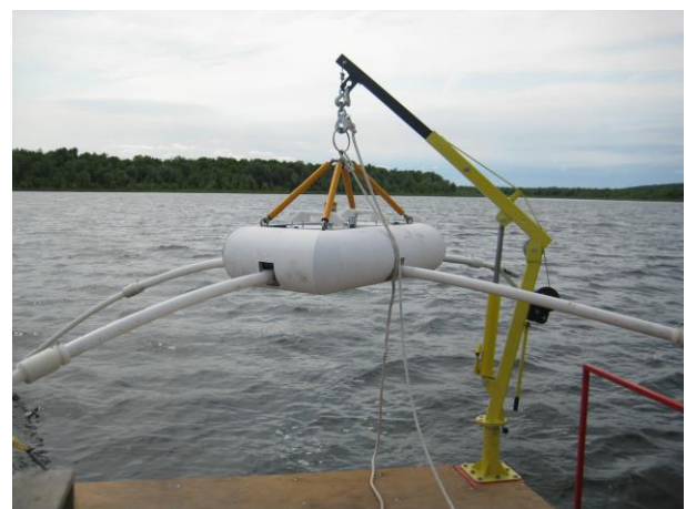
Figure 4. Deployment of SMMT system during marine EM survey.
