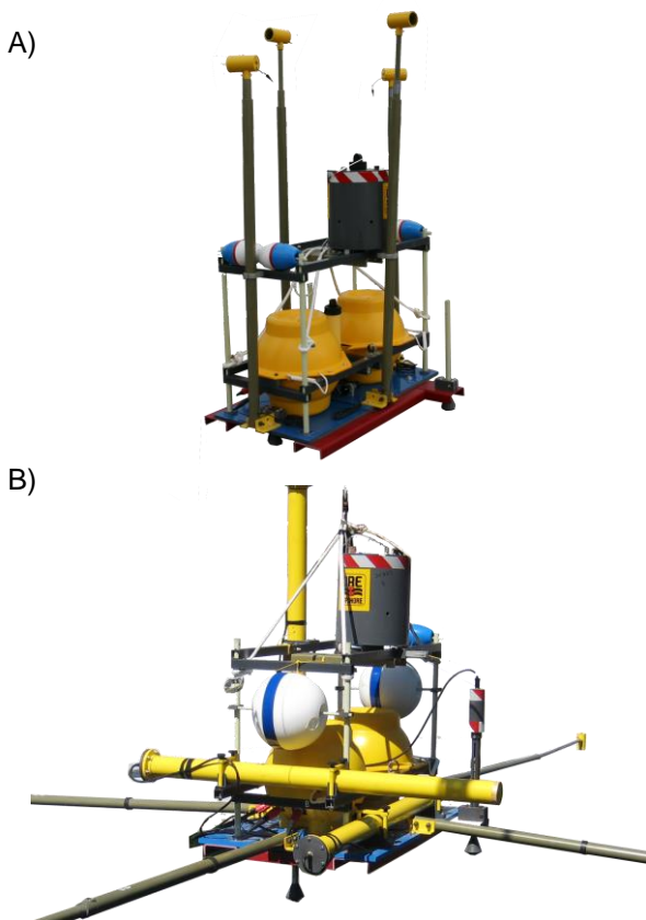
Figure 1. Marine EM receivers for coastal shelf exploration; A) 2-channel 2AUSS-07A; B) 5-channel 5AUSS-07A.
